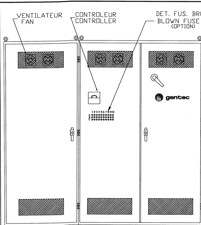
CABINET (PORTES FERMEES) ENCLOSURE (DOORS CLOSED)
