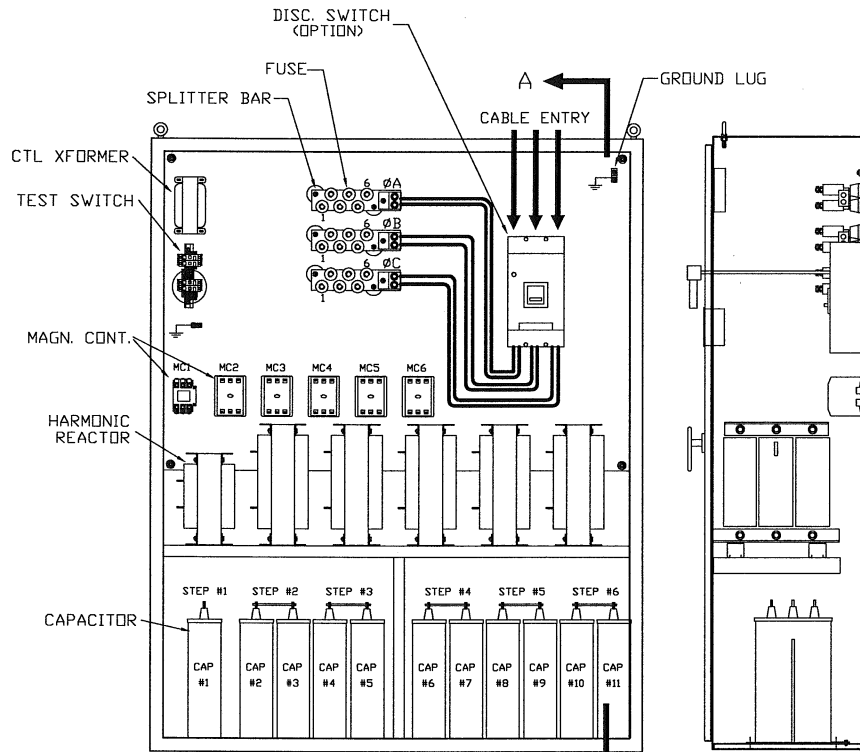
CUT VIEW
