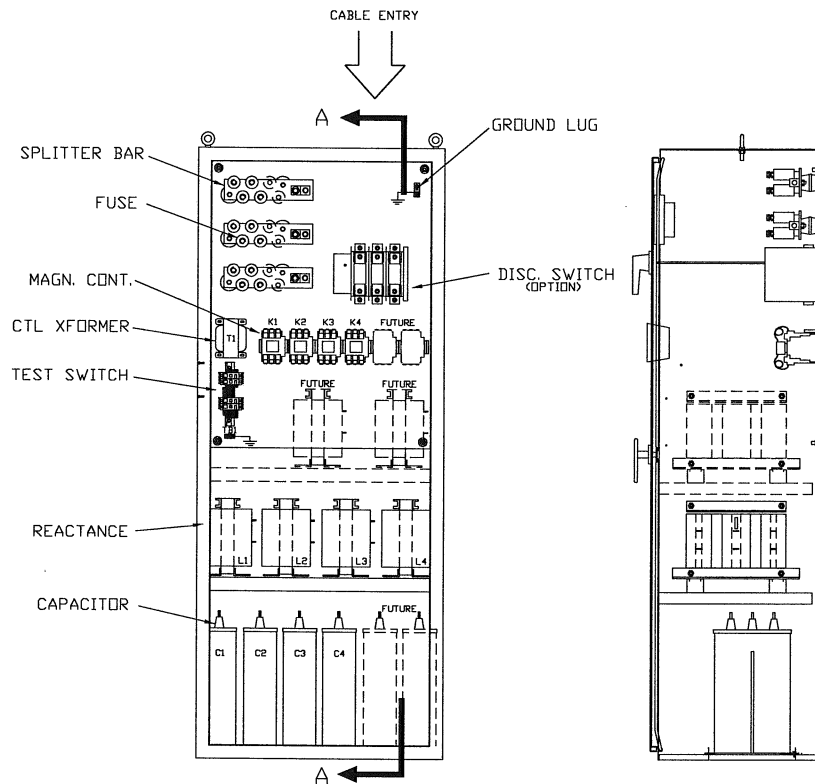
ENCLOSURE (DOOR OPENED)
