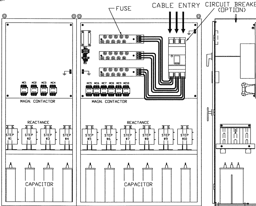
CUT VIEW
