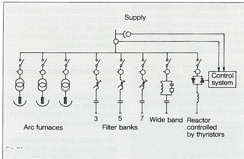
Fig. 24 Fast static compensator for arc furnaces.
