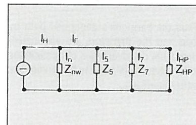
Fig. 22 Equivalent circuit of the harmonic filter and the network in accordance with Fig. 21.
