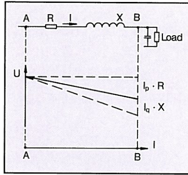
Fig. 5 Parallel compensation reduces the voltage drop.
