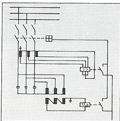
Fig. 19 Schematic diagram of an HV capacitor bank connected in star with unbalance protection.
