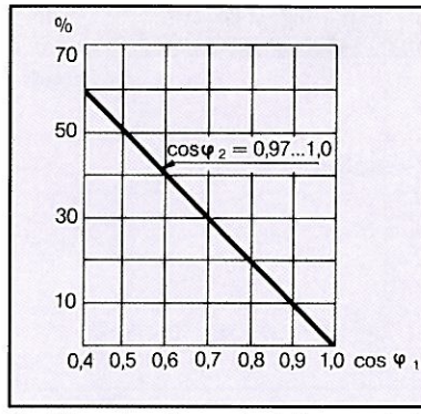
Fig. 3 Percentage decrease in design current of a network when the power factor ( \cos \varphi_2 ) is improved to near unity.
