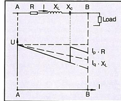
Fig. 6 Voltage may be raised to the desired level by means of a series capacitor
