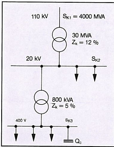
Fig.10 Schematic diagram of the example
