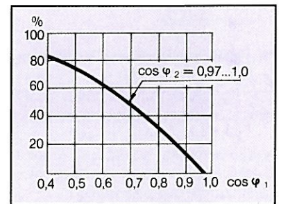
Fig. 4 Percentage decrease in total losses of a network with improvement in power factor.
