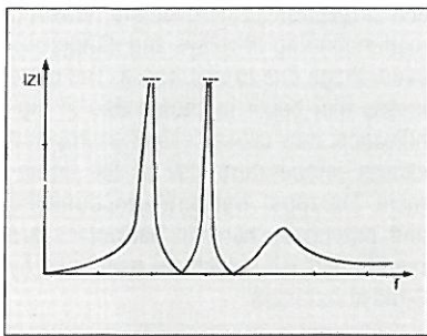
Fig. 23 Impedance curves of the harmonic filter and other network in accordance with figures 21 and 22.
