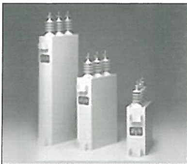
Fig. 17 One-phase high voltage capacitor units
