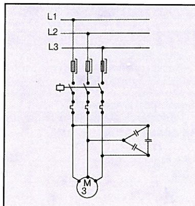
Fig. 7 Principle of individual motor compensation
