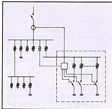
Fig.9 Connection scheme comprising fixed capacitors and automatically controlled capacitor bank.
