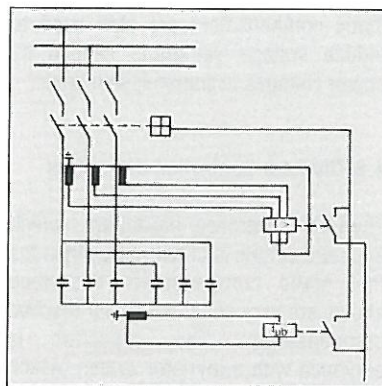
Fig. 20 Schematic diagram of an HV capacitor bank connected in double star with overload, short-circuit and unbalance protection
