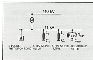
Fig. 21 Typical filter construction.
