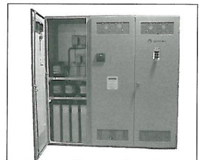
Fig. 15 Automatic capacitor bank with blocking reactors
