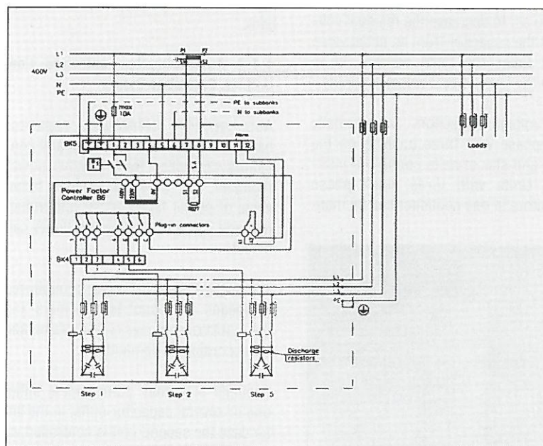
Fig. 16 Schematic diagram of an automatically controlled capacitor bank with power factor controller.
