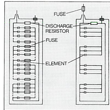
Fig. 18 Internally fused unit Externally fused unit
