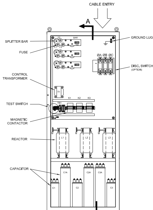
ENCLOSURE (DOOR OPENED)
