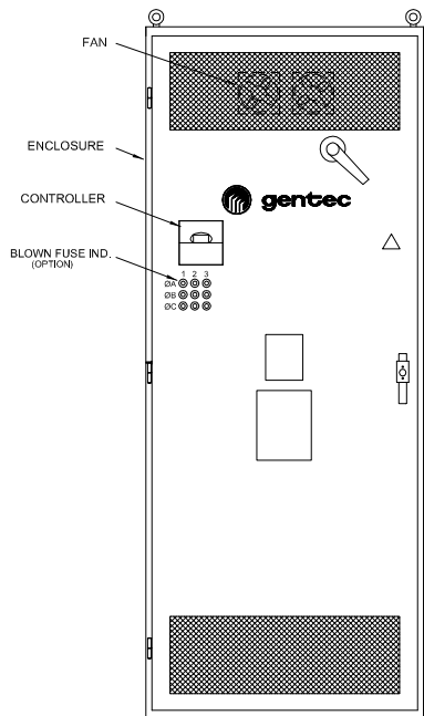
ENCLOSURE (DOOR CLOSED)
