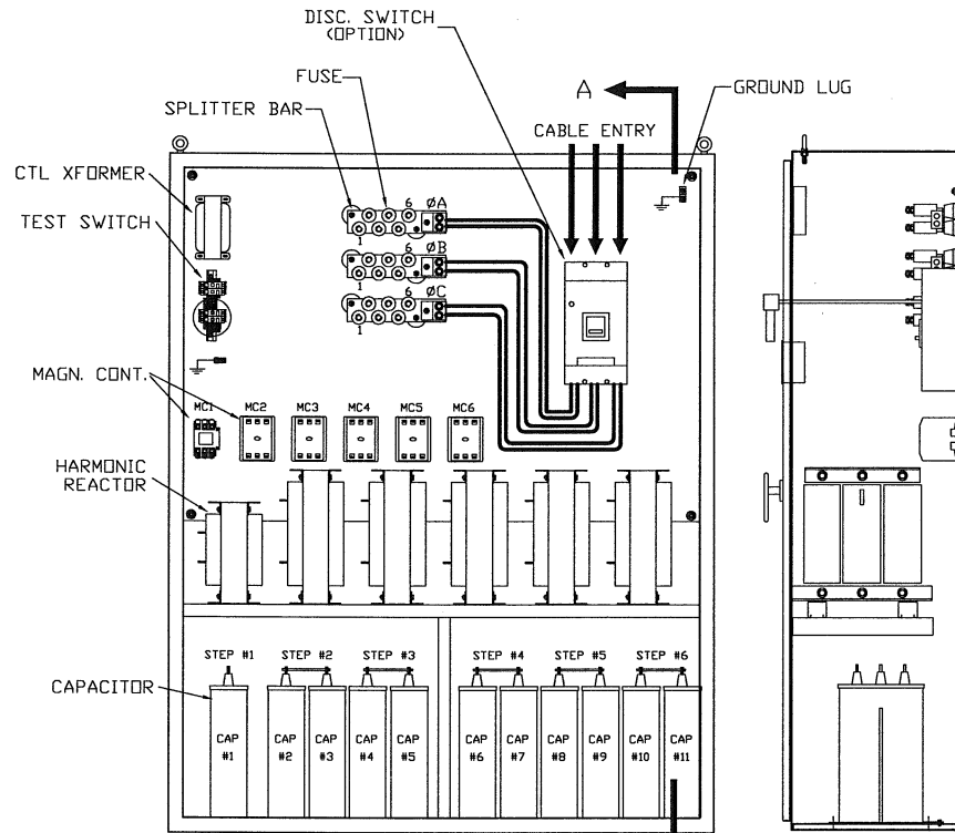
CUT VIEW
