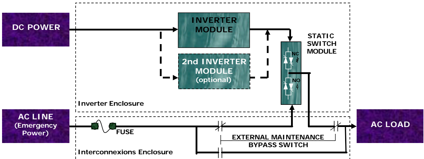
Single Line Diagram, OND3CS Series
