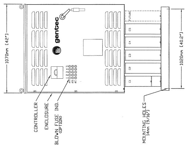
ENCLOSURE (DOOR CLOSED)
