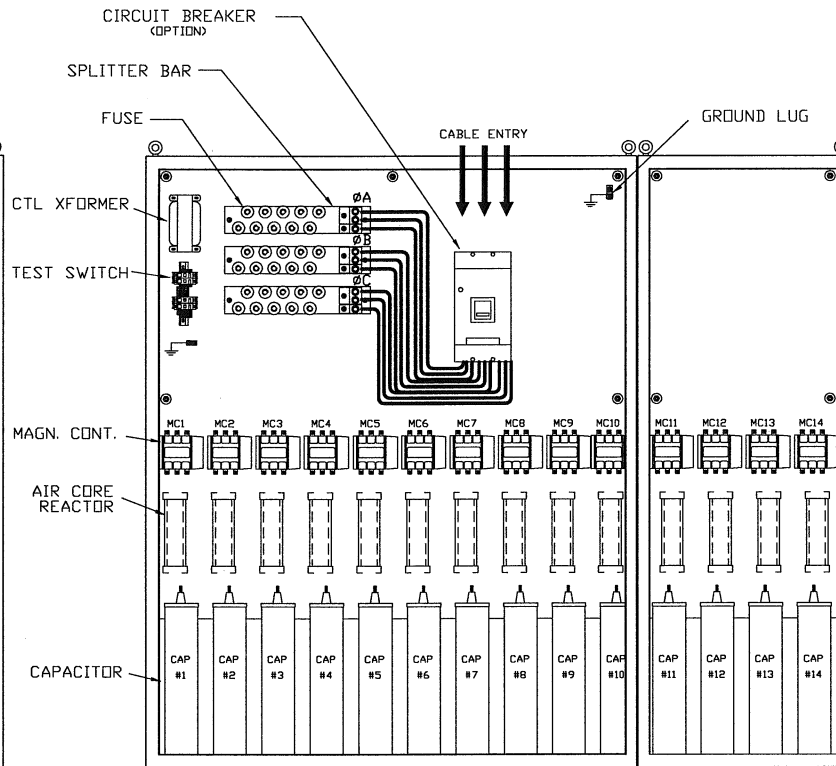
ENCLOSURE (DOORS OPENED)
