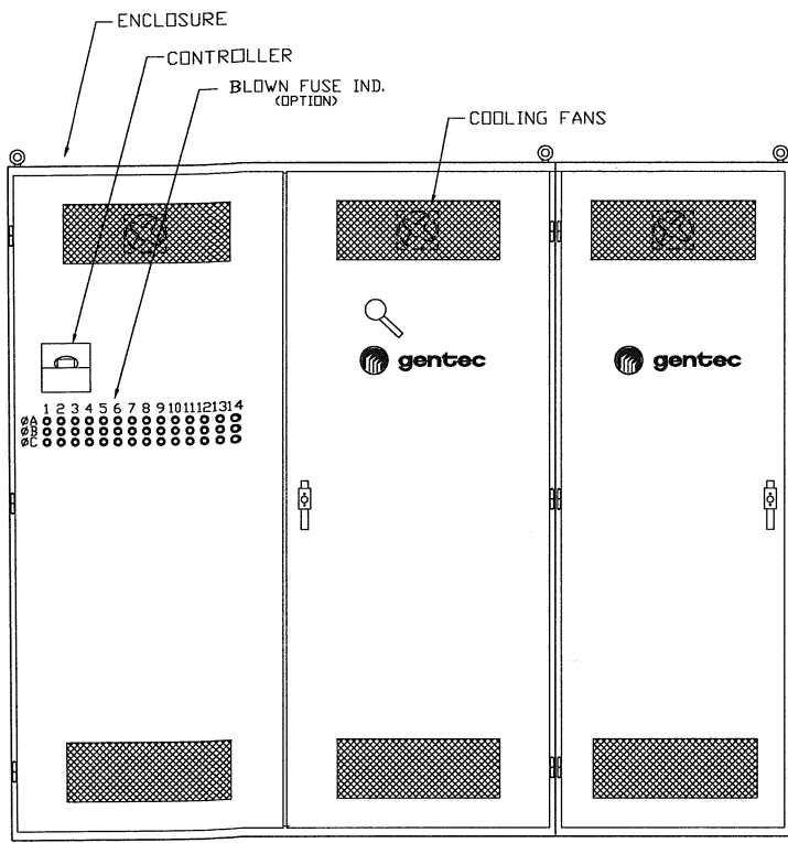
ENCLOSURE (DOORS CLOSED)
